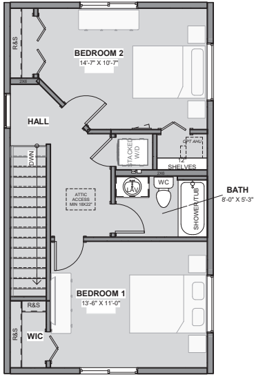
Level 2 - 18' Unit
